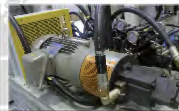
▲ Hydraulic set with low-noise, highly effective and less main-tenance. 高效能低噪音的油壓系統，故障率低。
